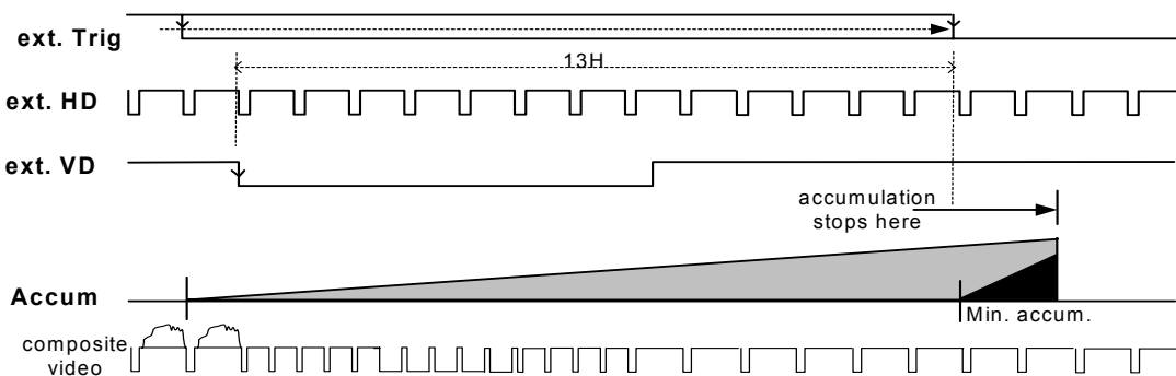
Fig. 26. Start/Stop timing details.
