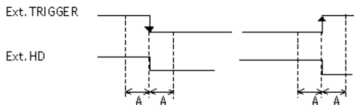
Fig. 14. Trigger/HD timing.
