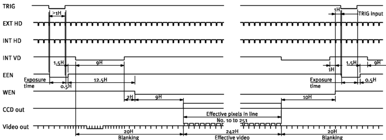
Fig. 20. Pulse width control EIA.
