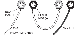
Figure 2. Series connection
