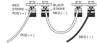
Figure 2. Series connection
