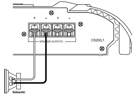
Figure 3. CS subwoofer amplifier with one woofer connection.
