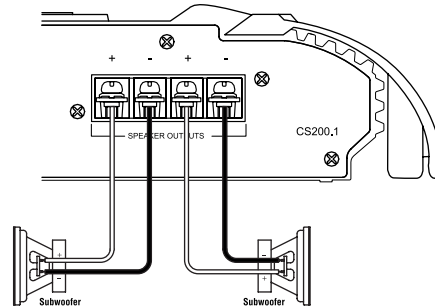
Figure 2. CS subwoofer amplifier with two woofer connections.
