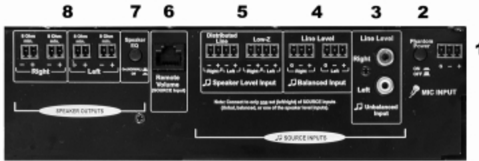
Figure 4b: Connector Panel
