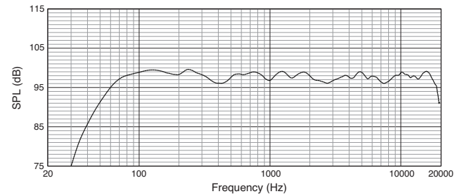
FREQUENCY RESPONSE (MONITOR)
