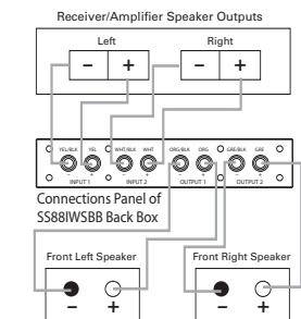
Connection Method #1, Using One SS881WS With Back Box (Remove Shorting Straps)
