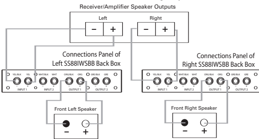
Connection Method #1, Using Two SS881WS Loudspeakers With Back Boxes (Use Shorting Straps)
