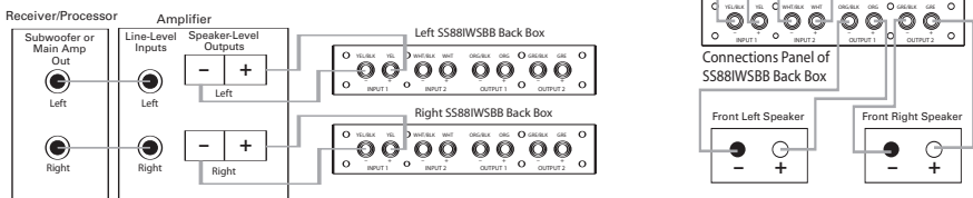
Connection Method #2, Using Two SS881WS Loudspeakers With Back Boxes (Use Shorting Straps)
