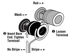
Figure 7. This example shows how to connect bare wires to the terminals.
