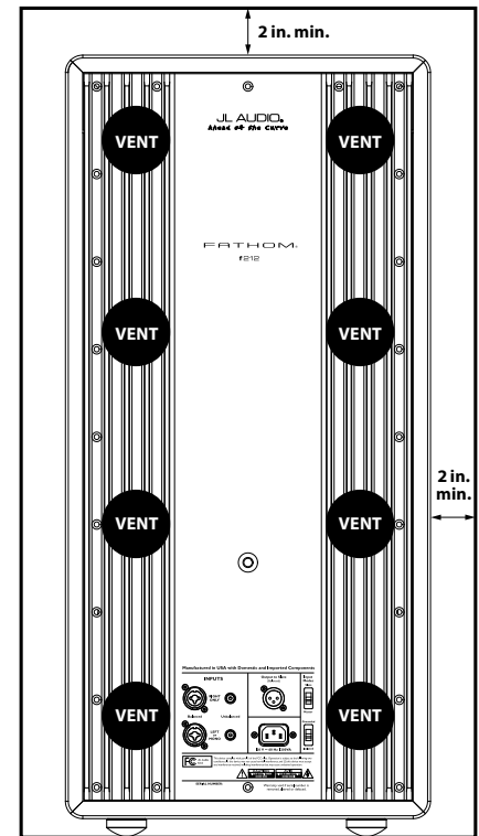
Rear-view of cabinet install:
