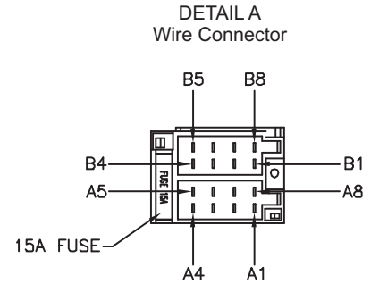
DETAIL A SHOWN FROM PIN VIEW
