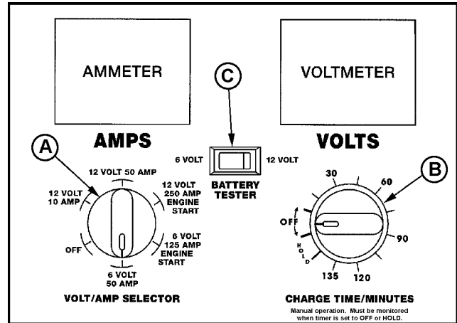
Control Panel
