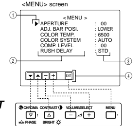
<Front panel buttons>
