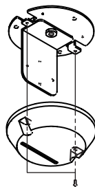
(2) Mount the cover on the bracket
