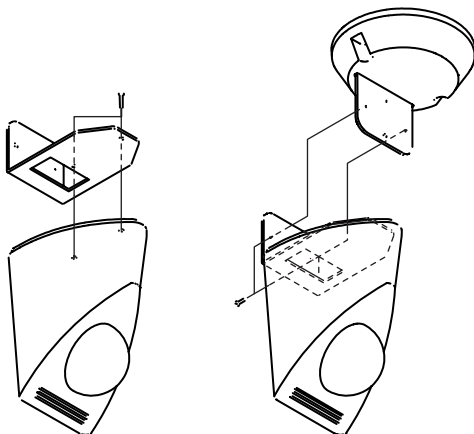
(3) Mount VN-C2U on the bracket
