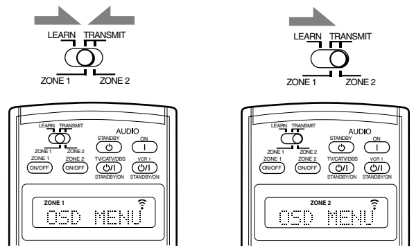
Ex. When you press TEXT DISPLAY with ZONE 1/ ZONE 2 (LEARN/ TRANSMIT) selector set to “ZONE 1.”
