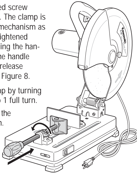
FIGURE 8. USING THE QUICK LOCK LEVER
