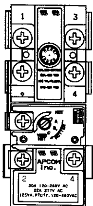
UPPER THERMOSTAT (DUAL ELEMENT MODELS ONLY)
