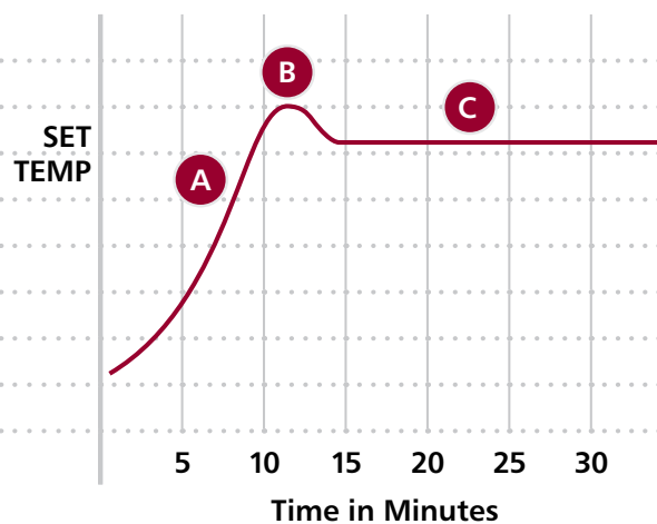
KitchenAid® Ovens with Even-Heat™ Preheat
