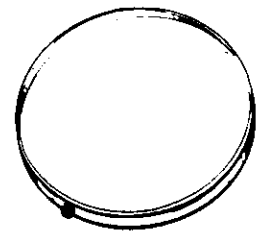
DRAIN PANS AVAILABLE IN 20" DIAMETER FOR WATER HEATERS HAVING A DIAMETER 18" OR LESS, 24" DIAMETER FOR WATER HEATERS HAVING A DIAMETER OF 22" OR LESS, AND AVAILABLE IN 28" DIAMETER FOR WATER HEATERS HAVING A DIAMETER 26" OR LESS
