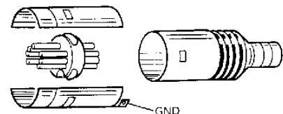
Internal wiring
