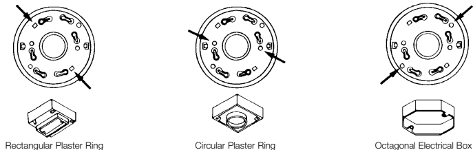
FIGURE 2. SELECT CORRECT MOUNTING HOLES ON TRIM RING
