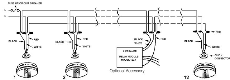
FIGURE 1 INTERCONNECT WIRING DIAGRAM
