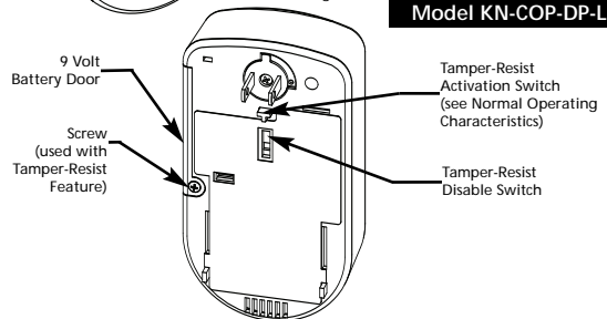
Model KN-COP-DP-LS
