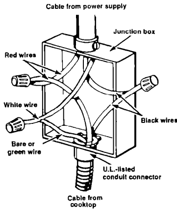
grounded neutral
