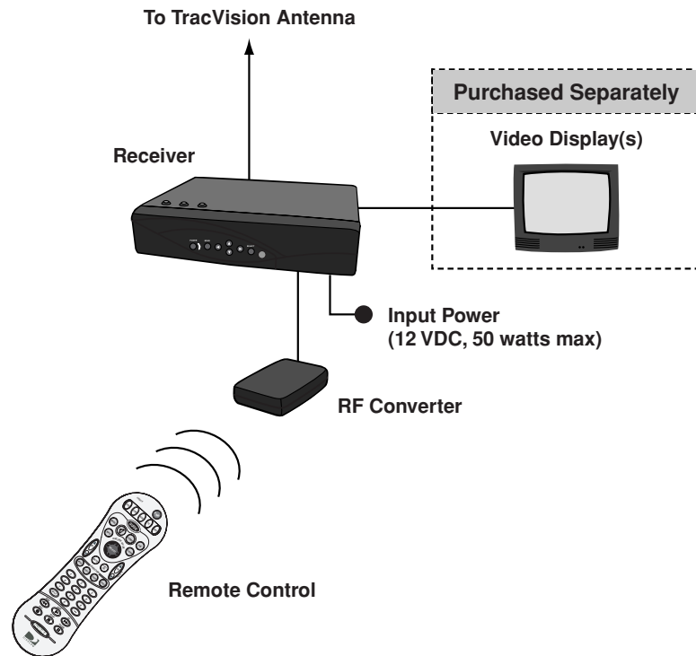
TracVision System Diagram (Typical Installation)
