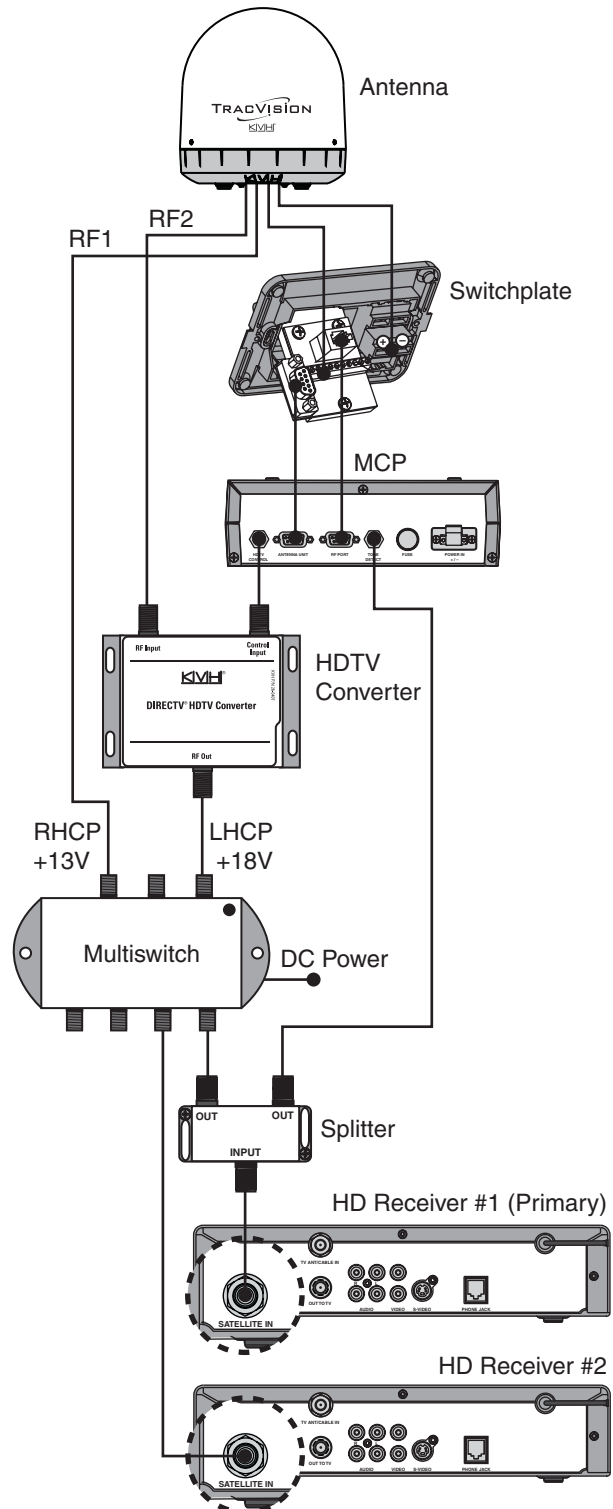
Figure 42: Wiring Multiple DIRECTV HD Receivers
