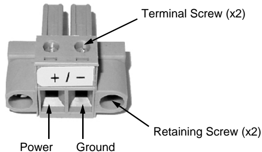
Figure 27: MCP Power Plug
