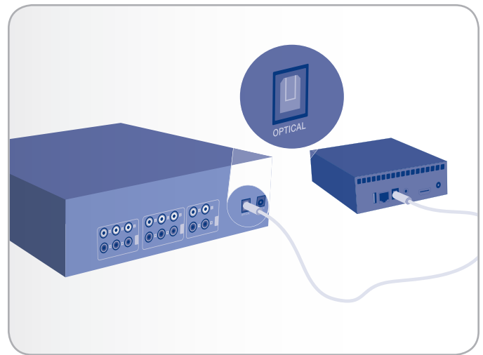
Fig. 17 - S/PDIF connection
