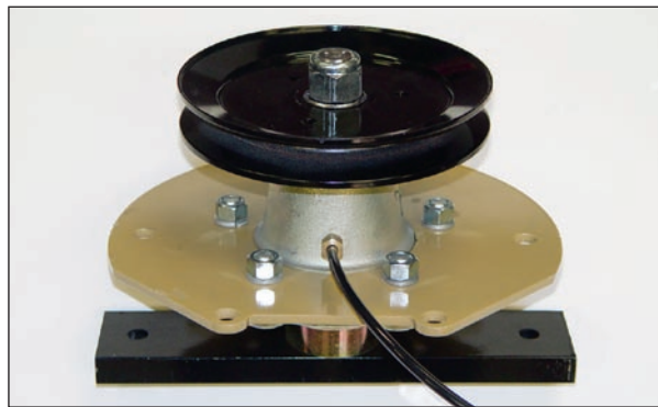
The commercial duty 1 3/8" blade spindle features a cast iron housing, additional steel plate support, a 3/4" thick blade support bar and a remote greasing line.
