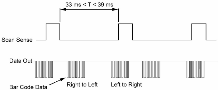
Figure 10: Timing Diagram
