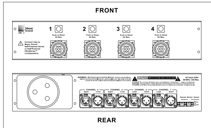
Figure 1.5. VIM-3 (top) and VIM-4 (bottom) modules
