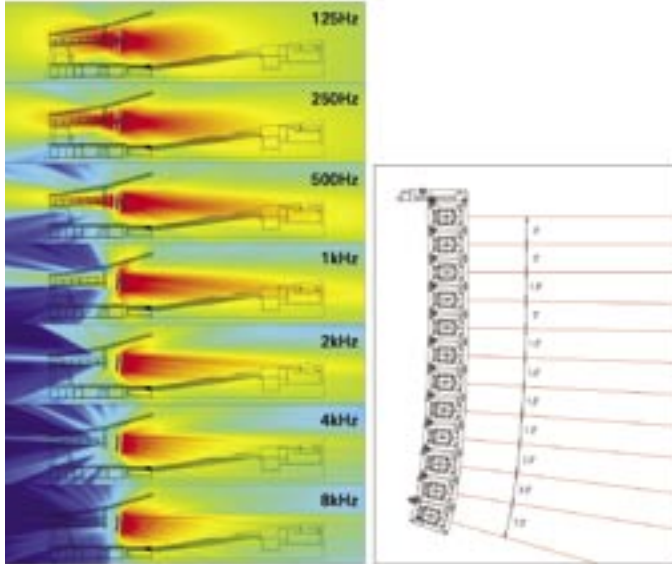
Figure 4.1: Using vertical splay to adjust a line array's coverage
