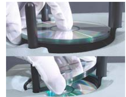
Fig. C - Loading Procedure
