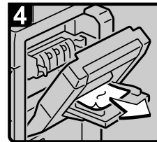
• Remove misfed paper from the bypass tray. • Close the duplex unit. • Close the bypass tray.
