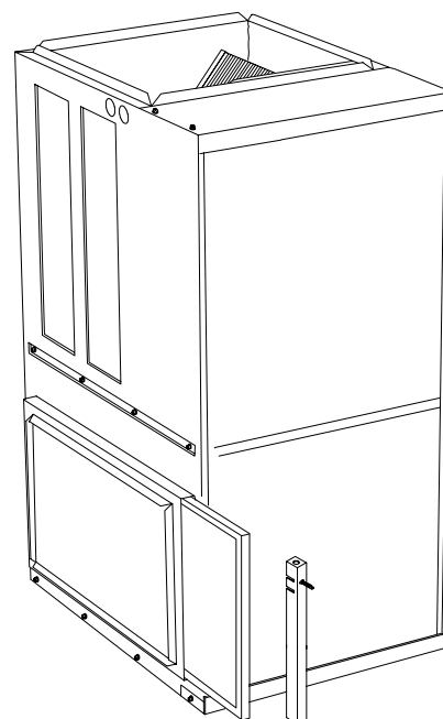
Internal Bottom Return Air Filter (Upflow shown)
