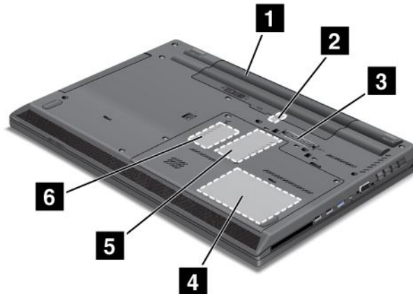
Figure 4. ThinkPad L430 and L530 bottom view
