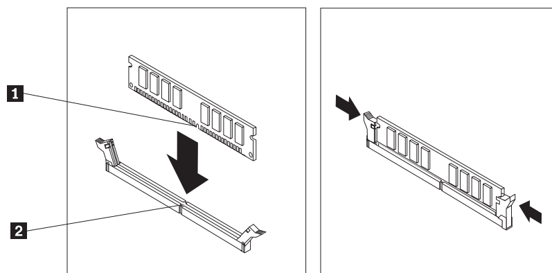
Figure 34. Installing the memory module
