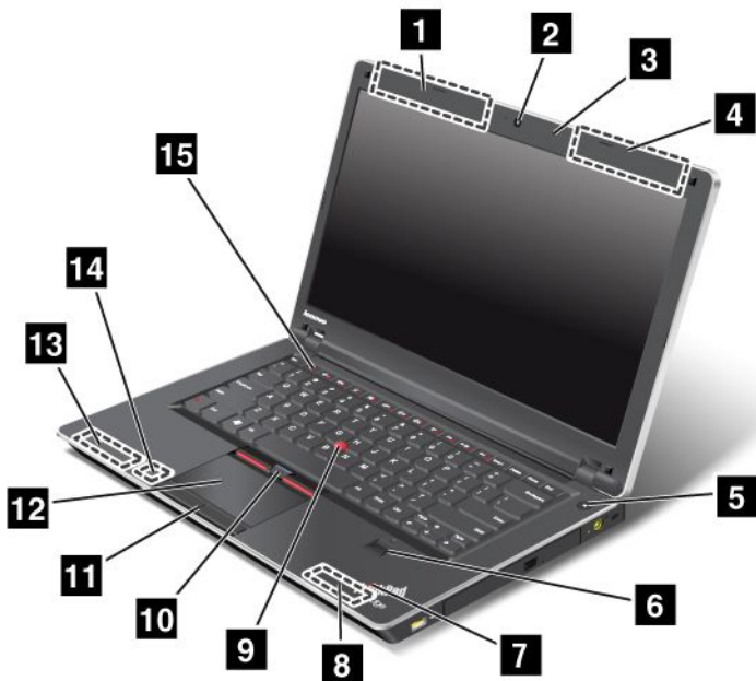
Figure 1. ThinkPad Edge E425 front view
