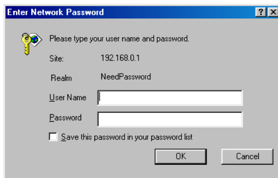
Figure 16: Password Dialog
