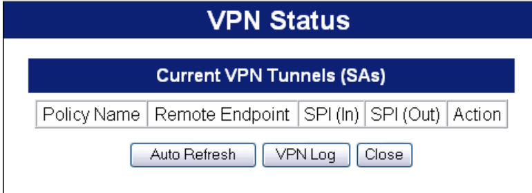
Figure 61: VPN-Status Screen
