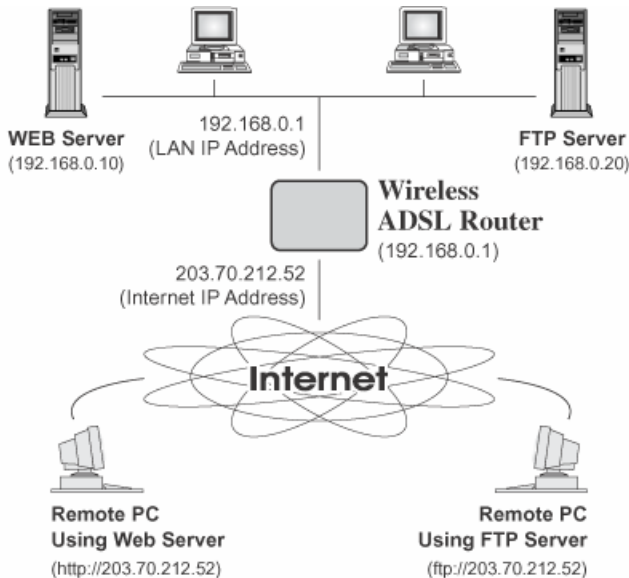
Figure 56: Virtual Servers
