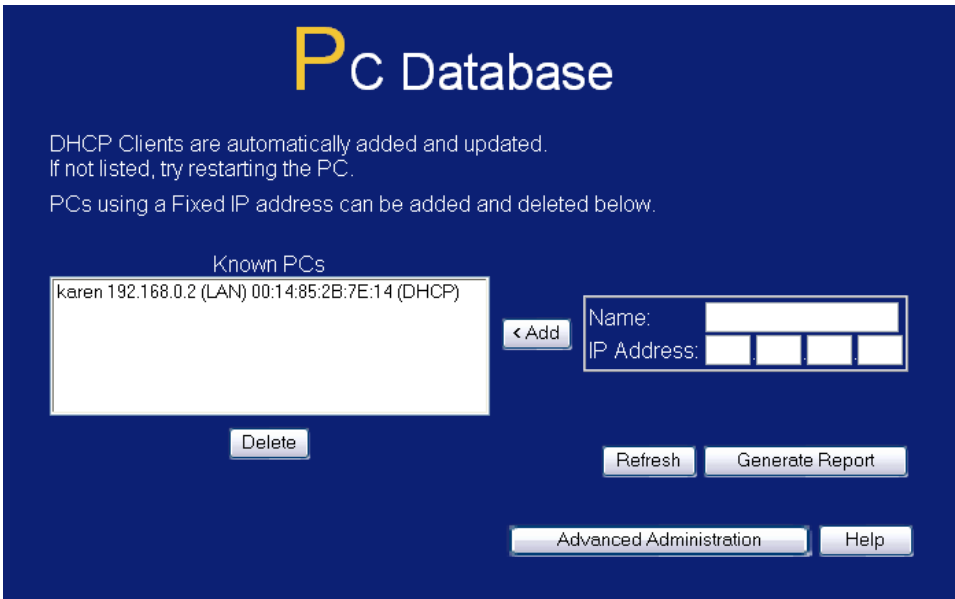
Figure 62: PC Database
