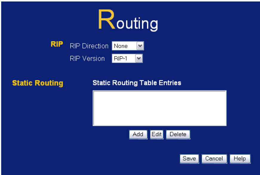
Figure 70: Routing Screen
