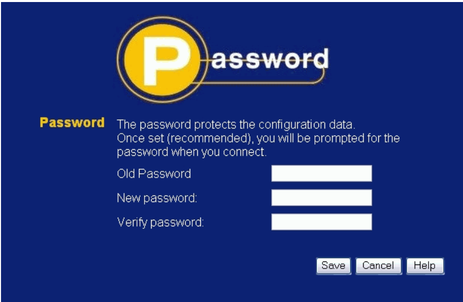
Figure 15: Password Screen
