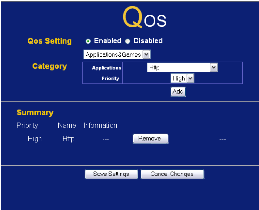
Figure 68: Qos Screen
