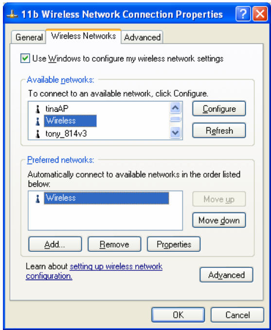
Figure 36: Preferred Networks
