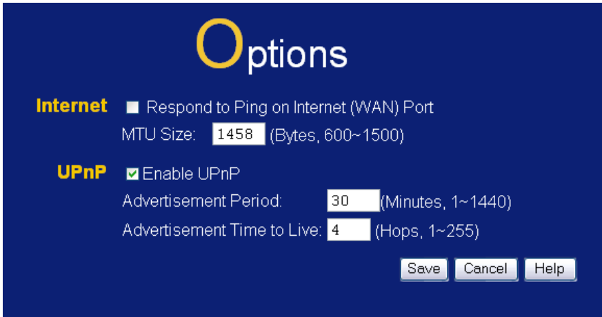
Figure 54: Options Screen
