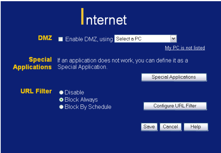
Figure 45: Internet Screen
