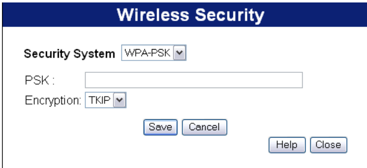
Figure 13: WPA-PSK
