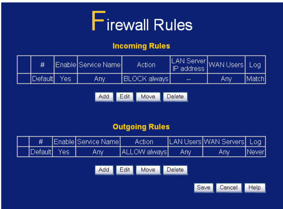
Figure 49 Firewall Screen
