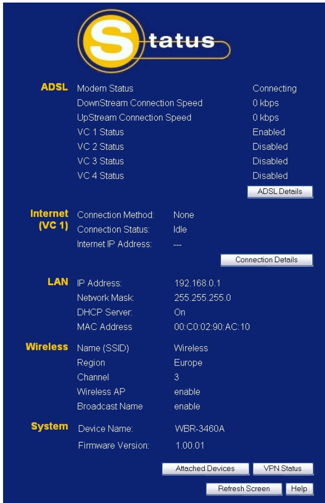
Figure 41: Status Screen
