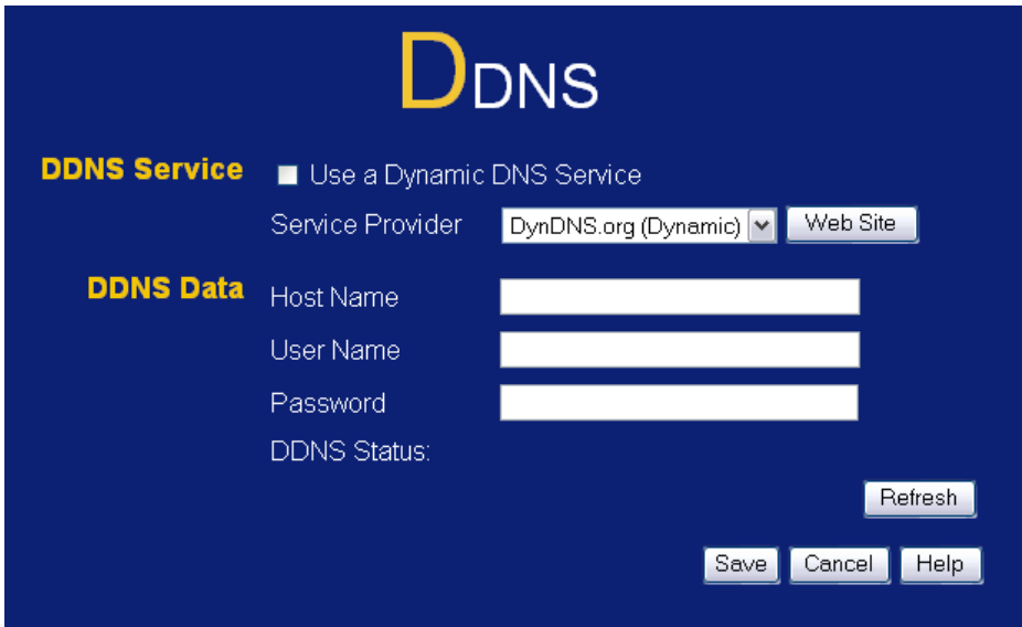
Figure 48: DDNS Screen
