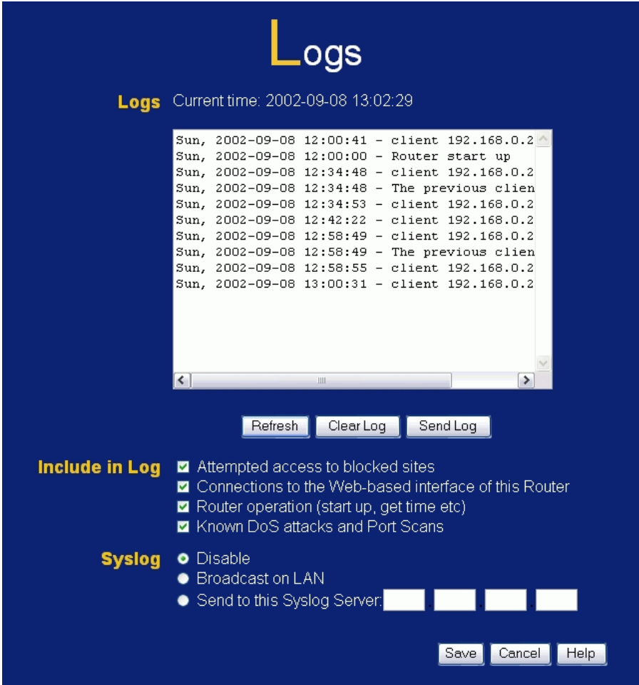
Figure 65: Logs Screen
