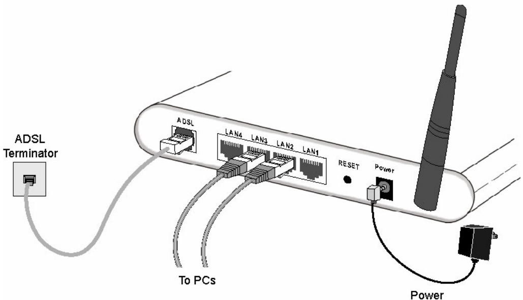
Figure 4: Installation Diagram
