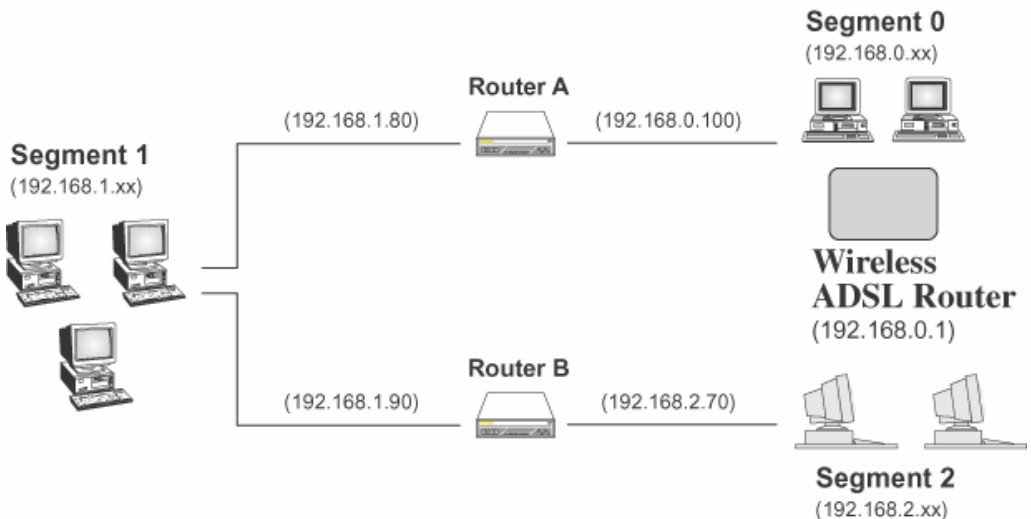
Figure 71: Routing Example
