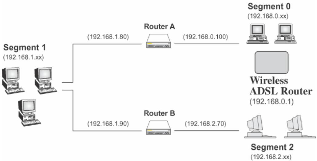
Figure 75: Routing Example
