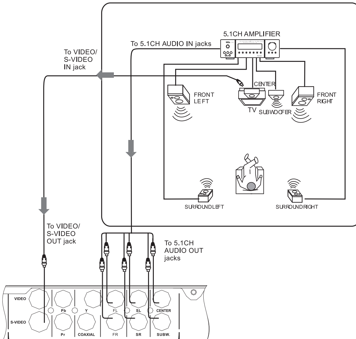
Connection Example
