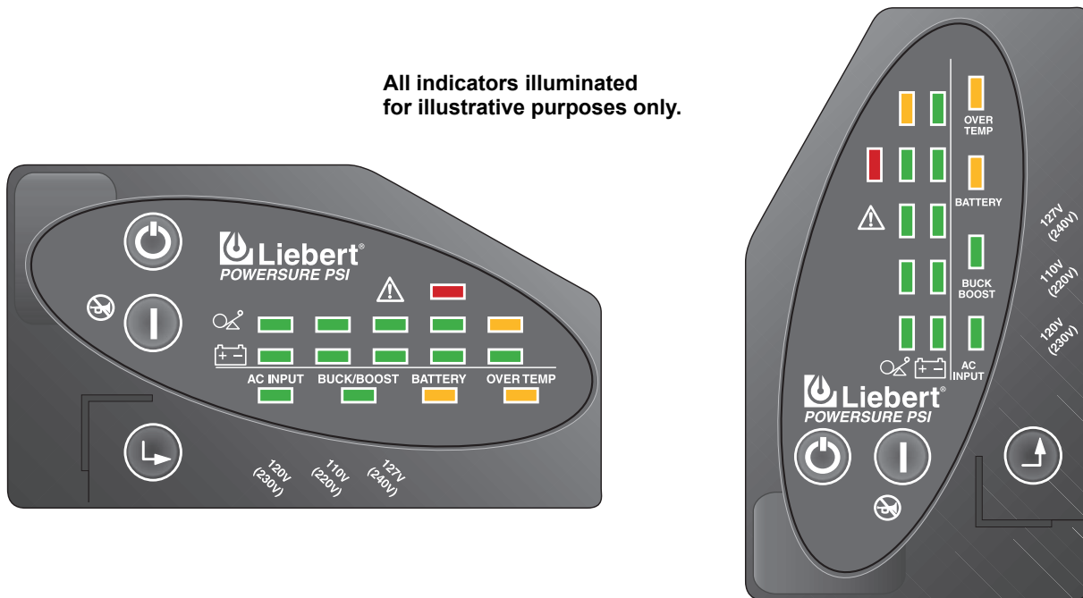
Figure 19 Status indicators
