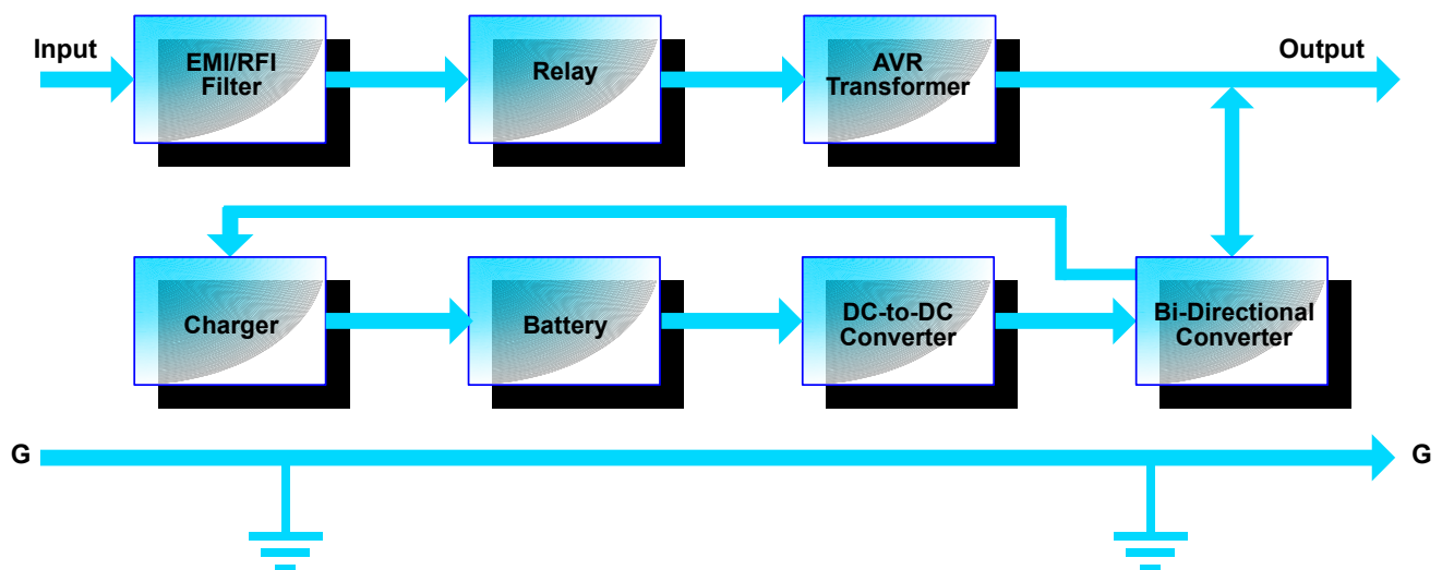
Figure 5 Line diagram of PowerSure PSI 2200VA & 3000VA
