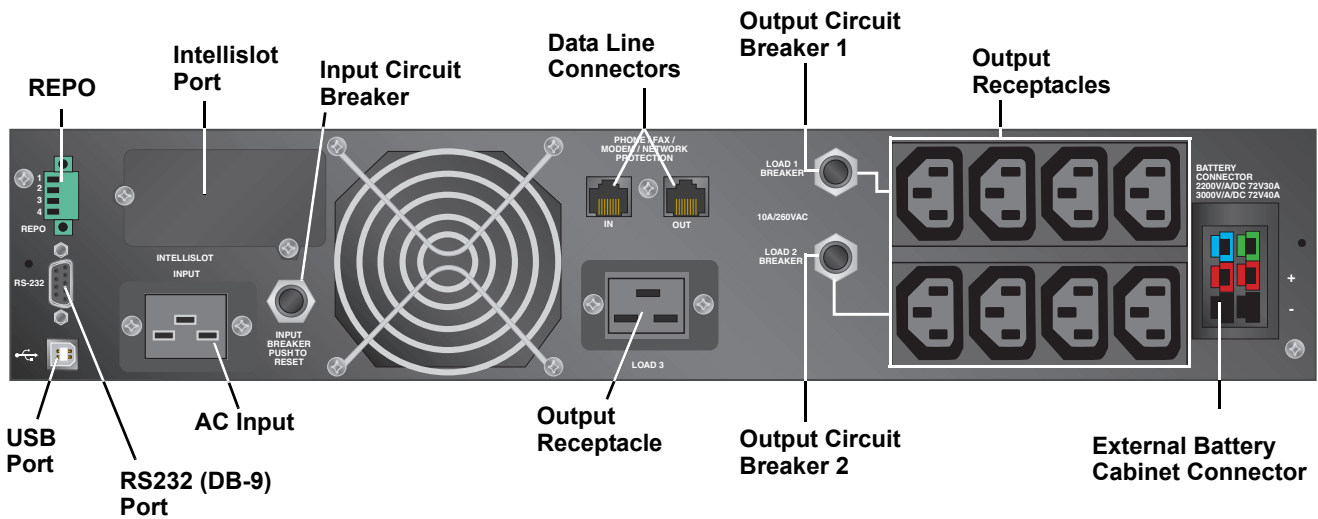
Figure 3 2200 and 3000VA PSI—rear view
