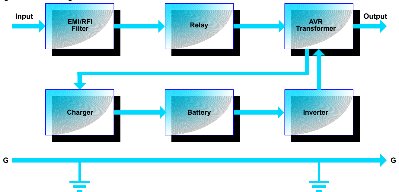
Figure 4 Line diagram of PowerSure PSI 1000VA & 1440VA
