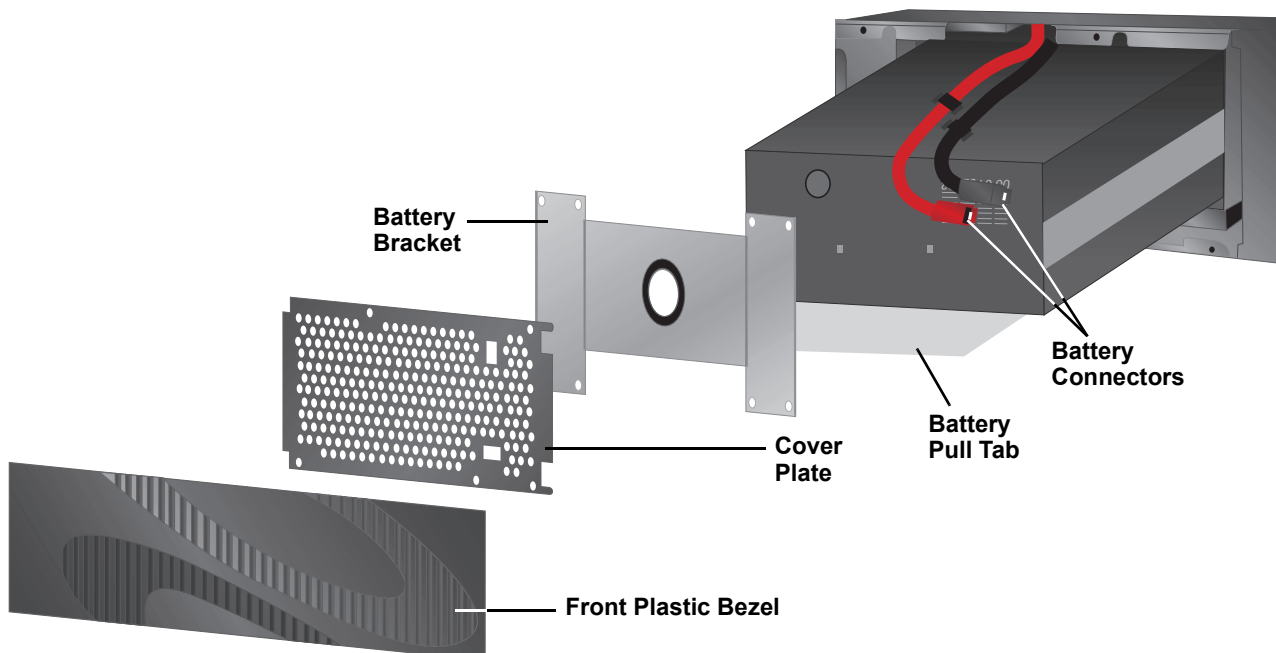
Figure 18 Battery replacement procedure
