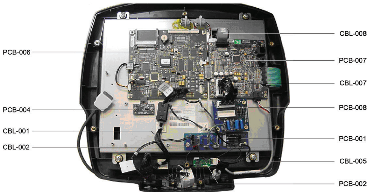
non-Treadmill Console
