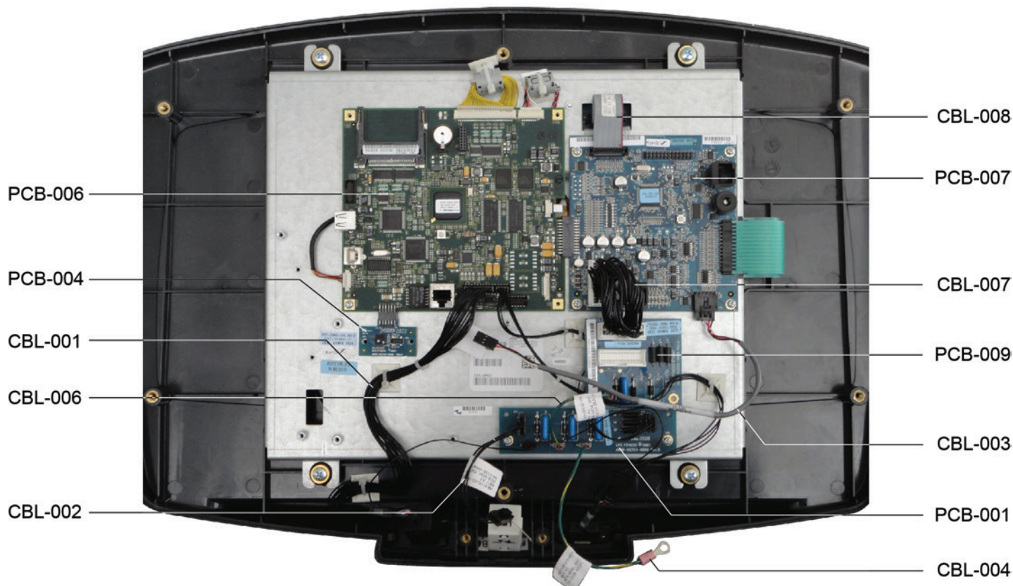
Treadmill Console
