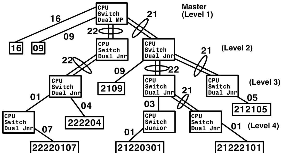
Fig. 6 - Creating menu entries for computers that are connected to cascaded LINDY CPU Switches
