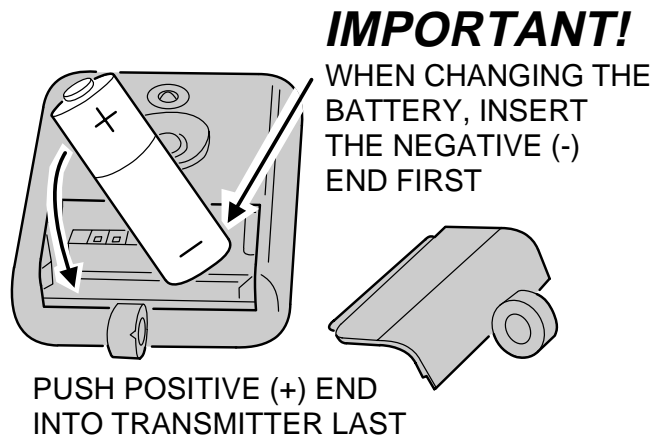
Figure 2. Proper Installation of Battery
