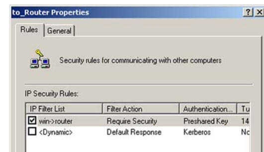
Figure B-18: Properties Screen
