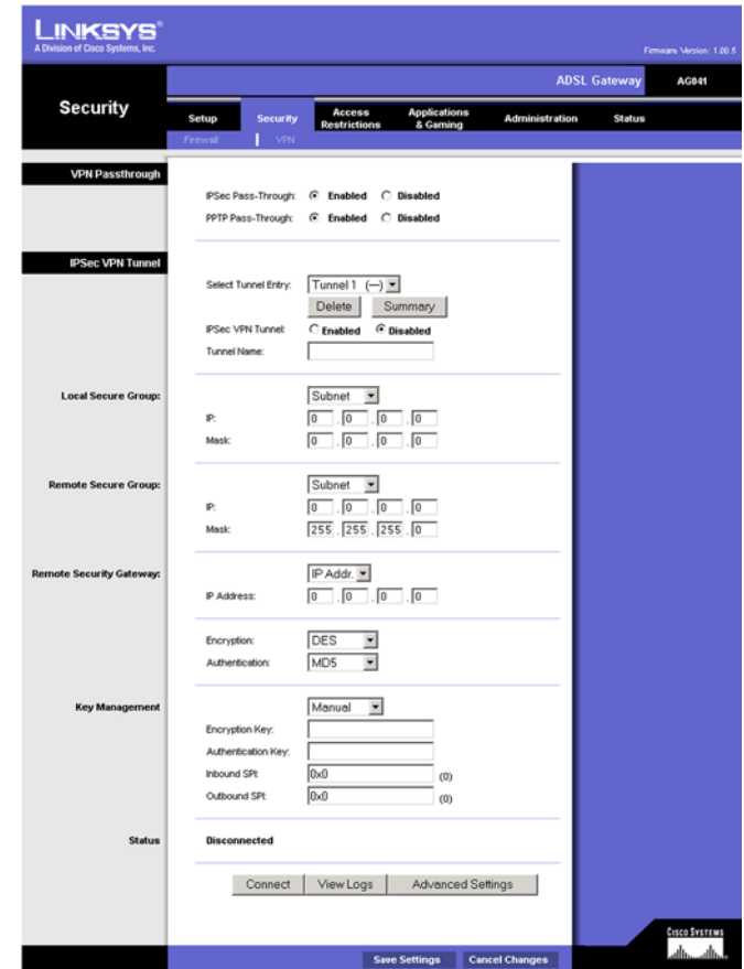
Figure 5-15: VPN with Manual Key Management
