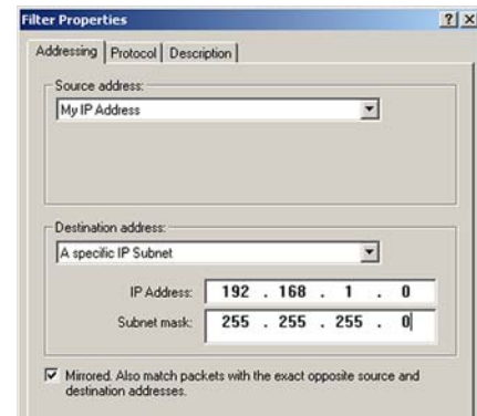
Figure B-8: Filters Properties
