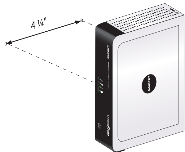
Vertical Mounting
