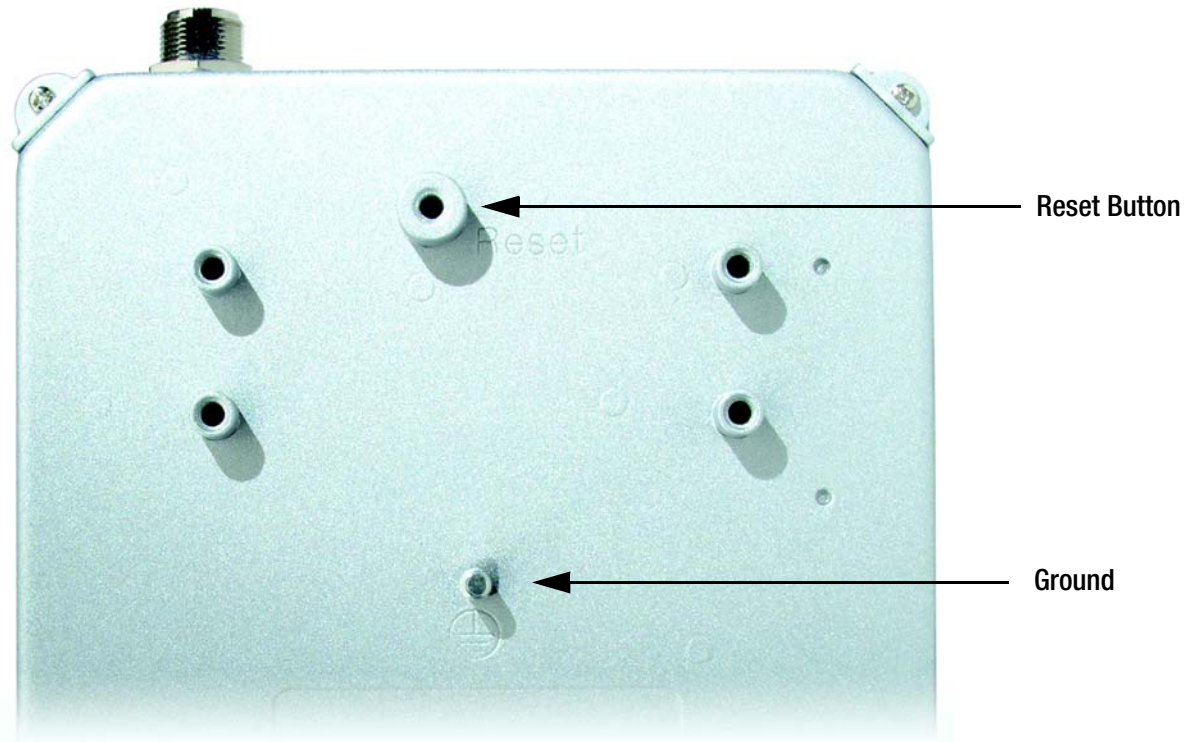
Figure 3-4: Back Panel
