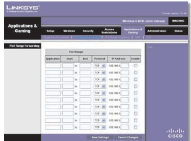
Applications and Gaming &gt; Port Range Forwarding
