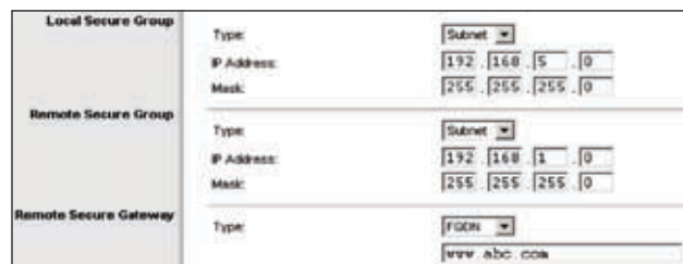
WRV200 IPsec VPN Settings
