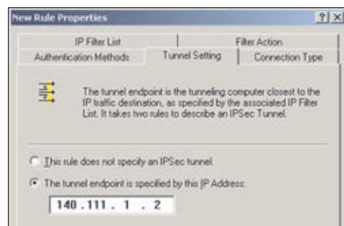
Tunnel Setting Tab
