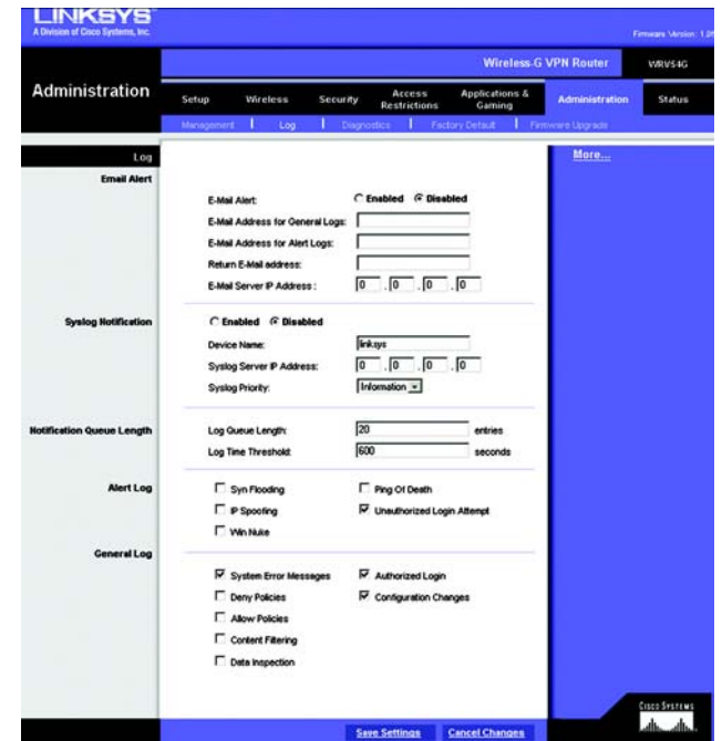
Figure 6-31: Log
