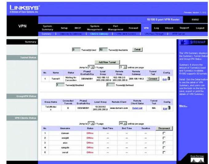
Figure 5-42: VPN Tab - Summary
