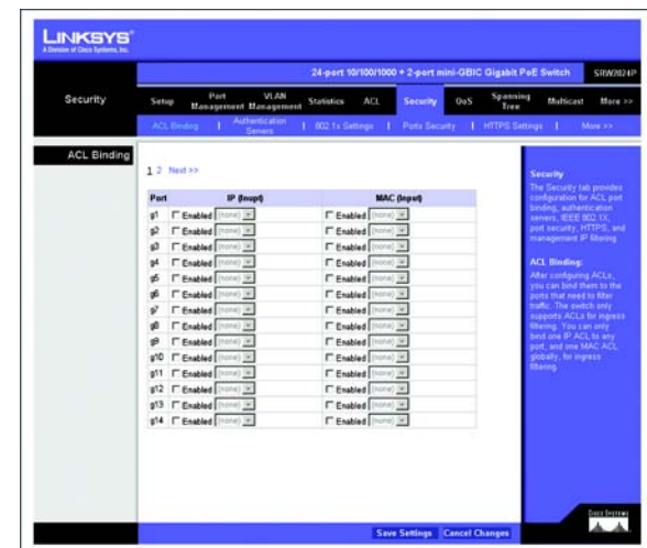
Figure 5-27: Security - ACL Binding
