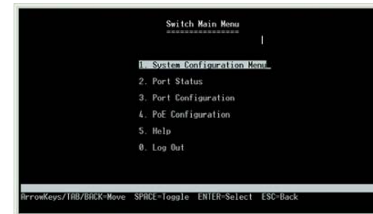
Figure 4-6: Switch Main Menu
