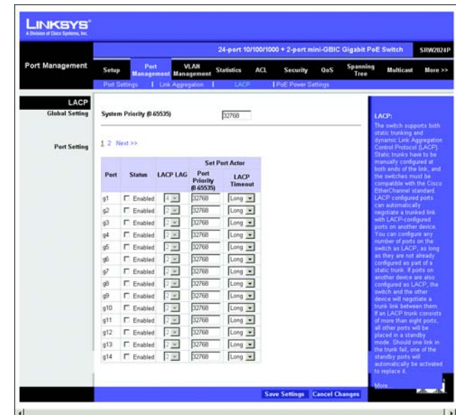
Figure 5-10: Port Management - LACP
