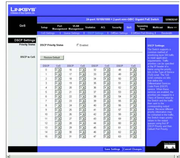
Figure 5-37: QoS - DSCP Settings
