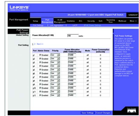
Figure 5-11: Port Management - PoE Power Settings
