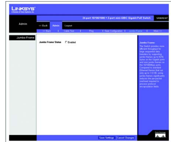
Figure 5-61: Admin - Jumbo Frame
