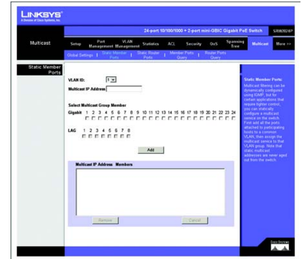
Figure 5-47: Multicast - Static Member Ports
