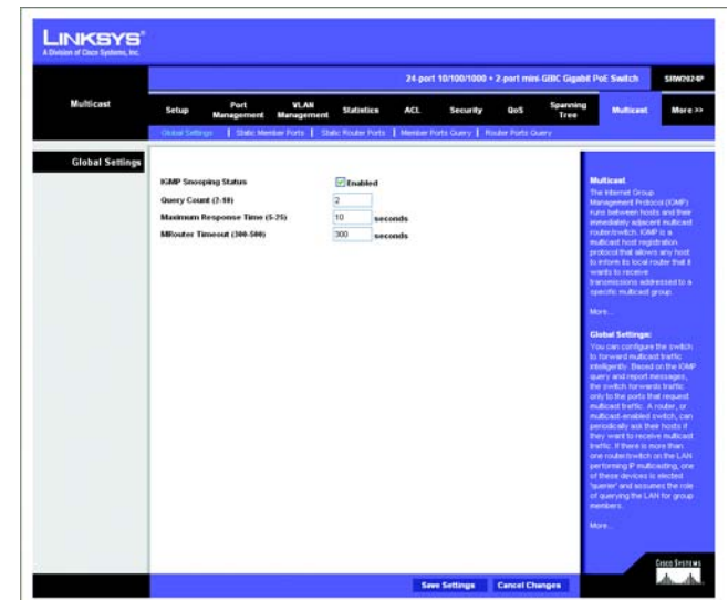
Figure 5-46: Multicast - Global Settings
