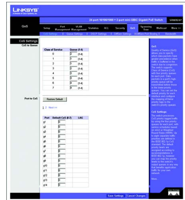
Figure 5-35: QoS - CoS Settings
