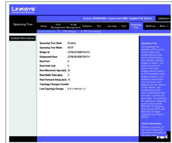
Figure 5-43: Spanning Tree - Global Settings
