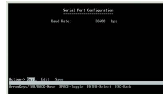
Figure 4-12: Serial Port Configuration
