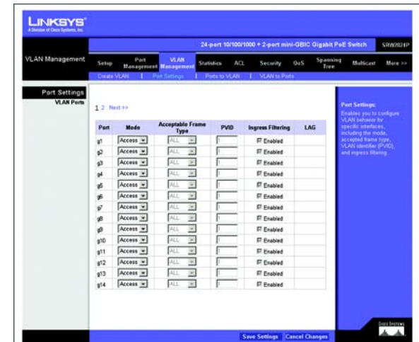
Figure 5-13: VLAN Management - Port Settings
