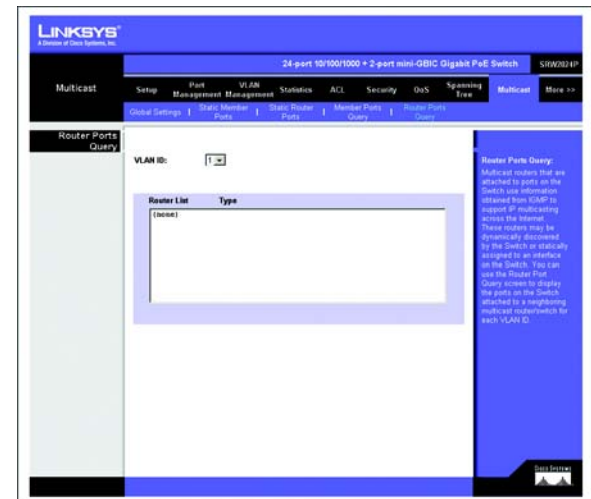
Figure 5-50: Router Ports Query
