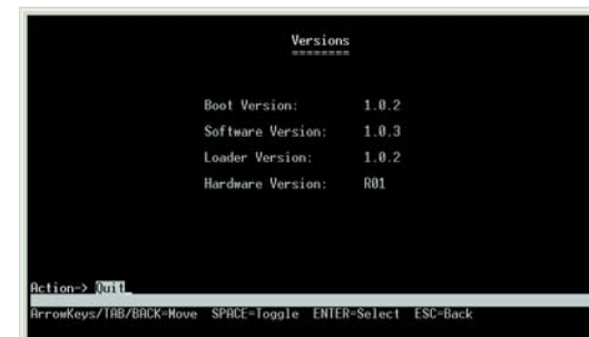
Figure 4-8: System Information Menu
