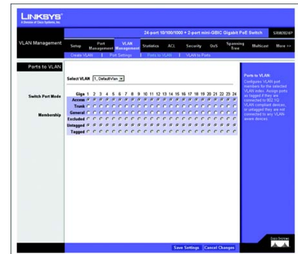
Figure 5-14: VLAN Management - Ports to VLAN
