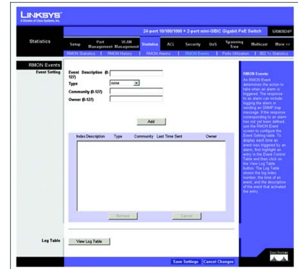
Figure 5-21: Statistics - RMON Events
