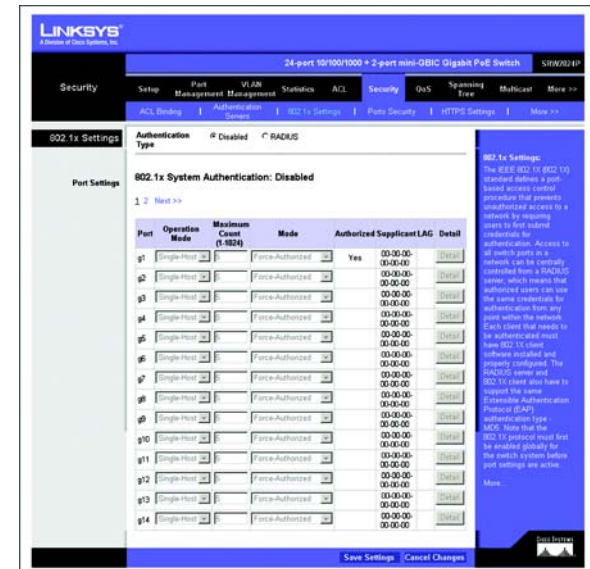
Figure 5-29: Security - 802.1x Settings
