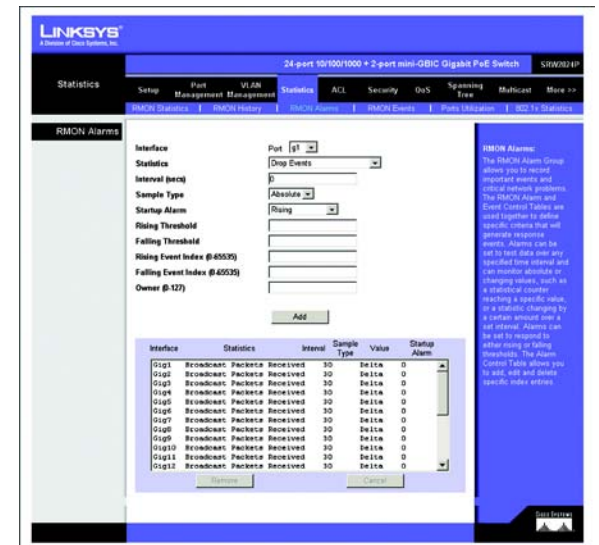
Figure 5-20: Statistics - RMON Alarm
