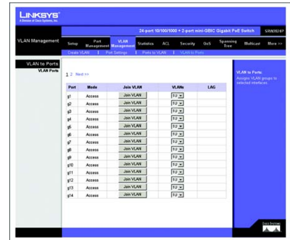
Figure 5-15: VLAN Management - VLAN to Ports
