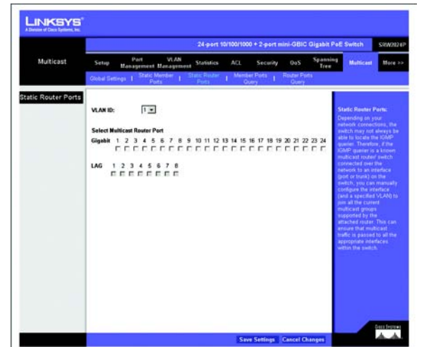
Figure 5-48: Multicast - Static Router Ports
