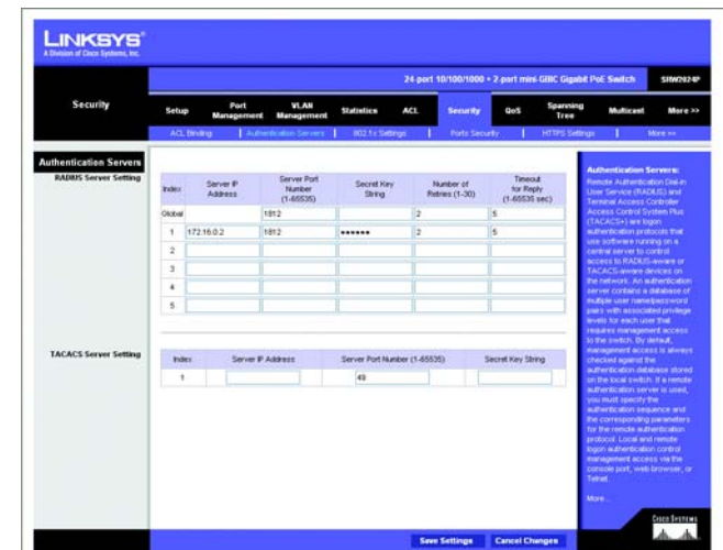
Figure 5-28: Security - Authentication Servers
