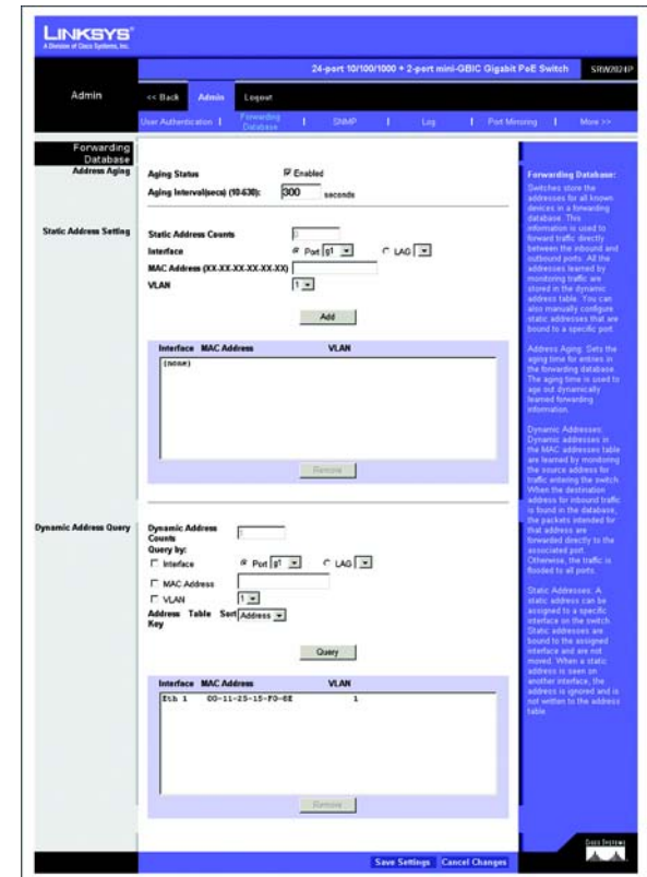
Figure 5-52: Admin - Forwarding Database
