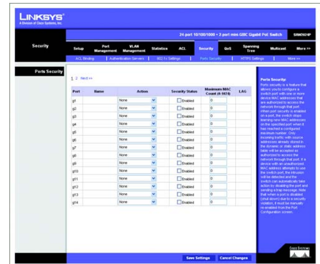
Figure 5-30: Security - Ports Security
