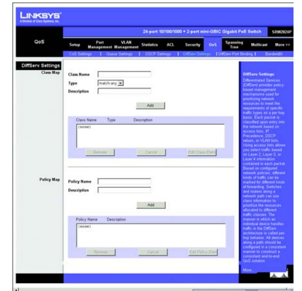
Figure 5-38: QoS - Diffserv Settings
