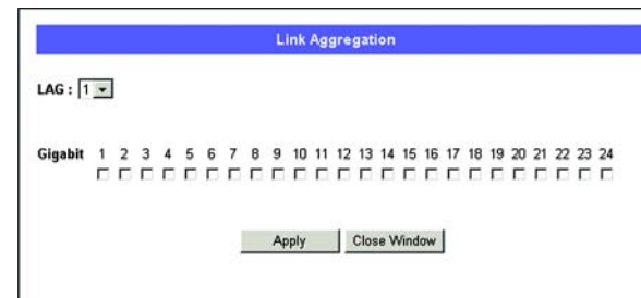
Figure 5-8: Link Aggregation - Link Aggregation Select Member
