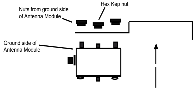
Diagram G. Reversing the Antenna Module on the Mounting Bracket.
