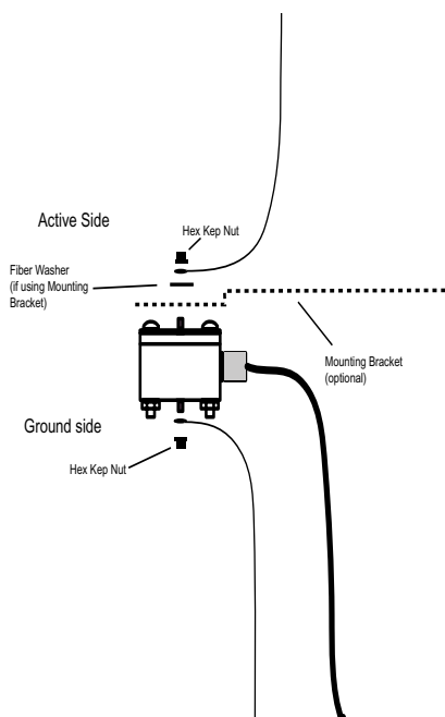
Diagram D. Flexible Dipole connection to the Antenna Module.
