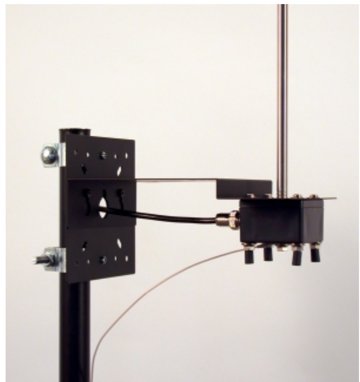
Using half of a flexible dipole for grounding a rigid dipole. This is a good choice when you don't have room to fully extend the ground side of the dipole.
