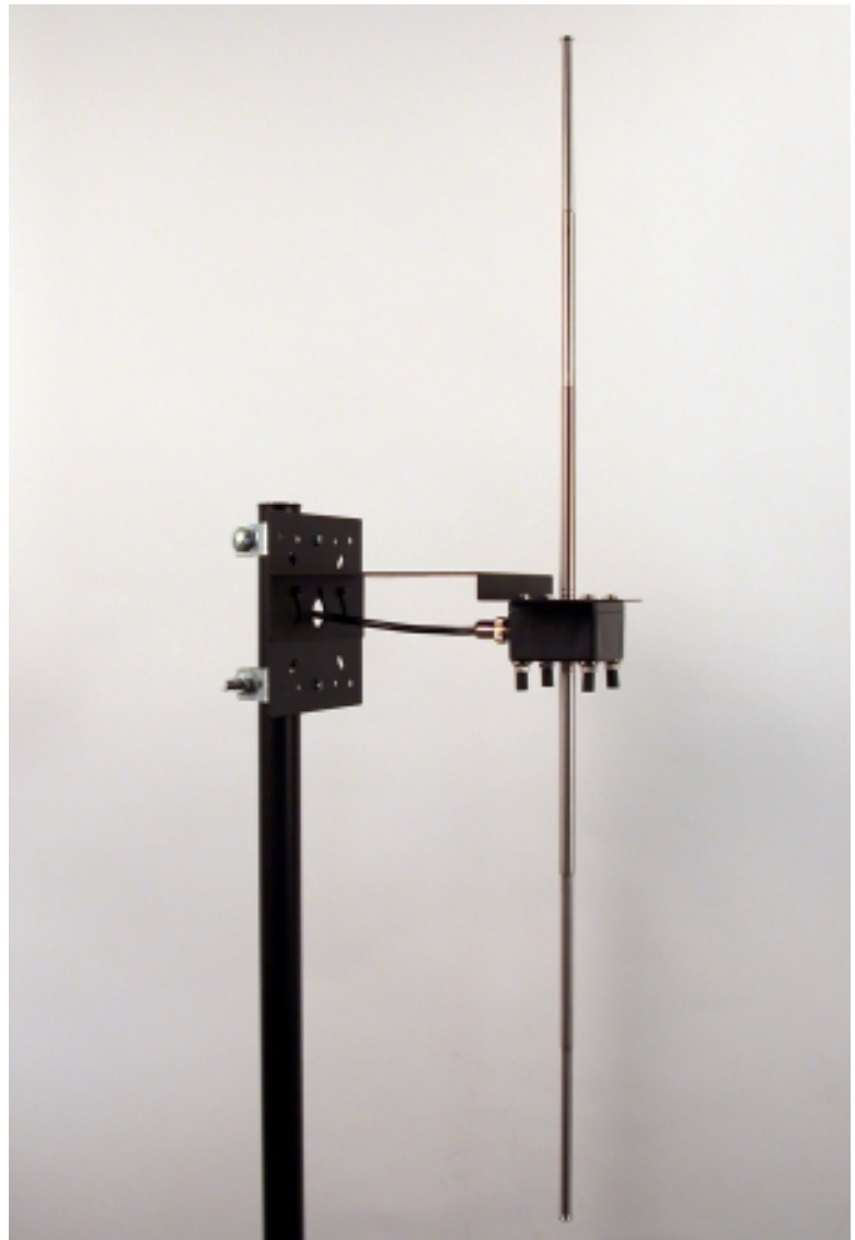
Installation of a dipole antenna on a vertical mast with the Mounting Plate. Note that the antenna is installed at the TOP of the mast.
