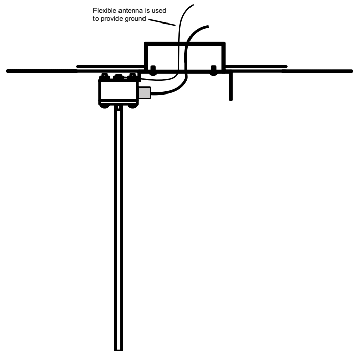
Diagram I. Ceiling mounted monopole with a flexible antenna attached to provide a ground. This installation creates a dipole antenna, which has better performance than a monopole. The Shorting Plate is not used in this configuration.
