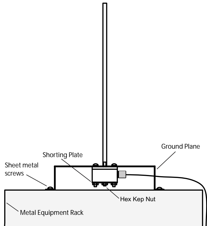
Diagram K. Mounting a Monopole on a metal surface.
