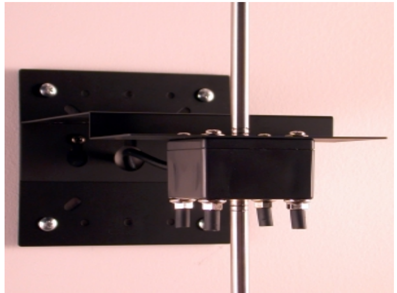
Rigid dipole sections screw onto the opposite sides of the antenna module, and are then fully extended.
