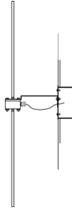
Diagram B. The Electrical Box mount uses the Mounting Plate and Mounting Bracket as shown above.
