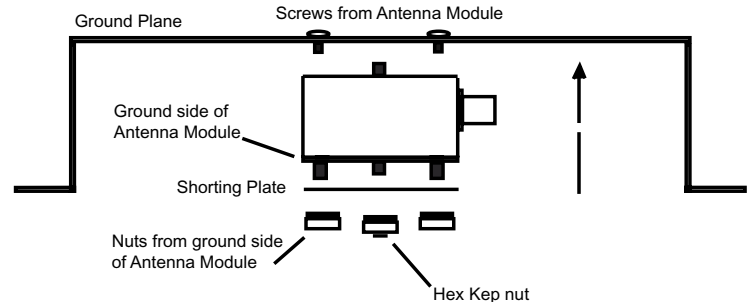
Diagram J. A reversed Antenna Module with Ground Plane and Shorting Plate.
