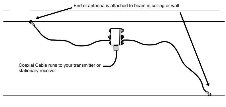
Diagram E. A flexible dipole can be mounted in your ceiling or wall as shown here. Although the Mounting Bracket is not shown here, it would be used to secure the Antenna Module to a beam.
